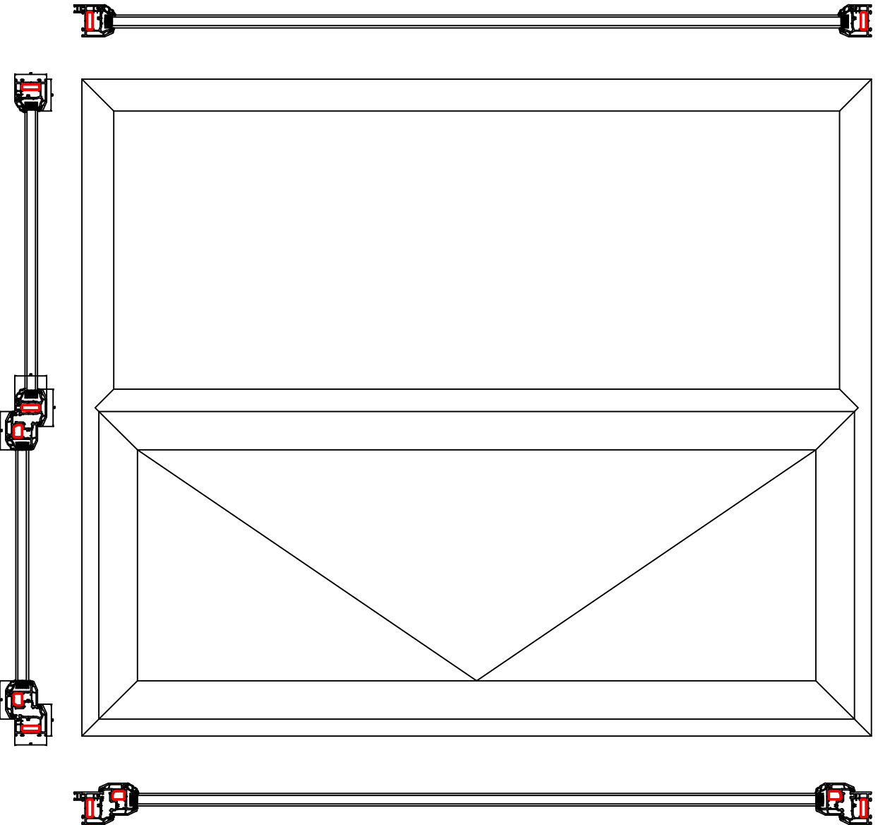
Cork Plastics Externally Glazed Window
