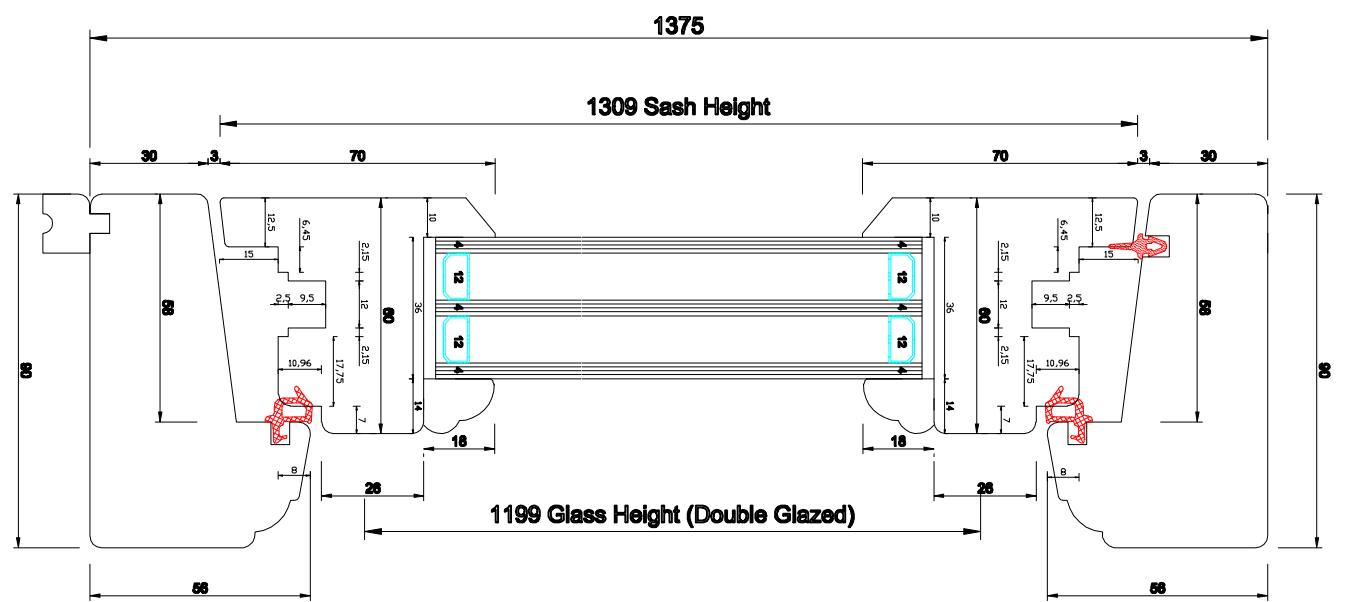
Section:B:B
